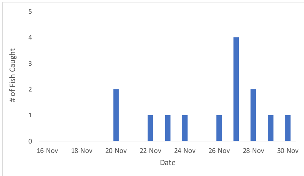
Figure 25. Chinook Captured Per Day 11/16/2023 to 11/30/2023 (Cougar Dam Head of Reservoir).
