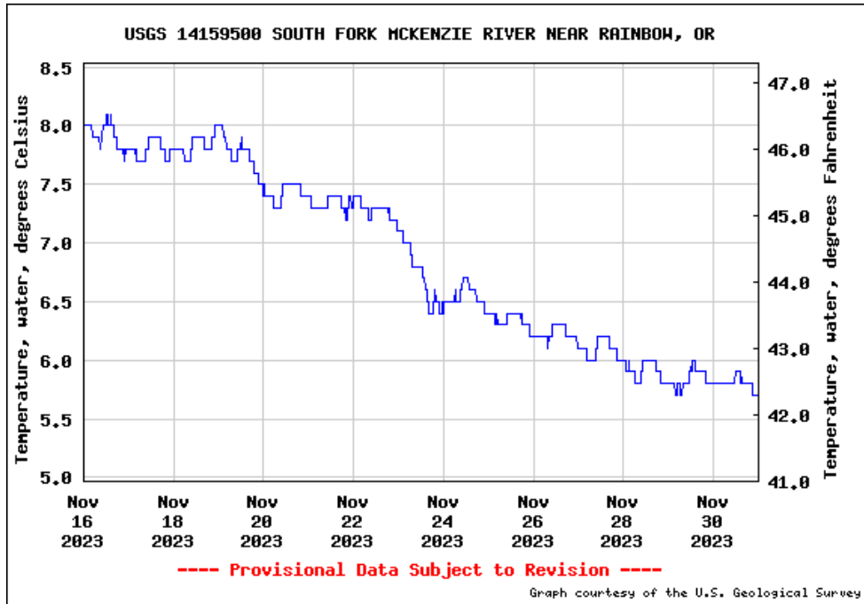
Figure 23. Temperature at PWR RST (Cougar Dam).
