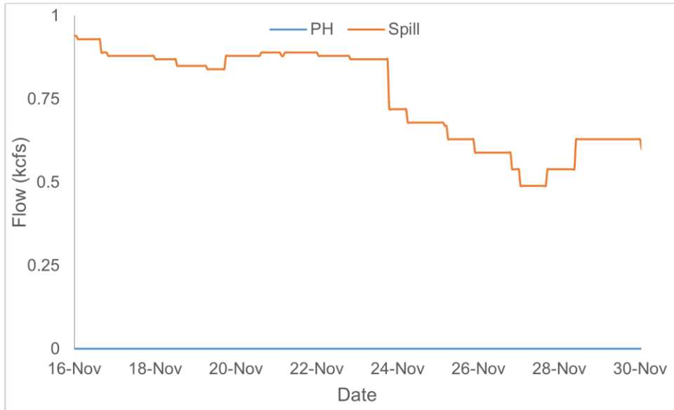
Figure 13. Hourly Flows PWR vs. Spill (Green Peter Dam).
