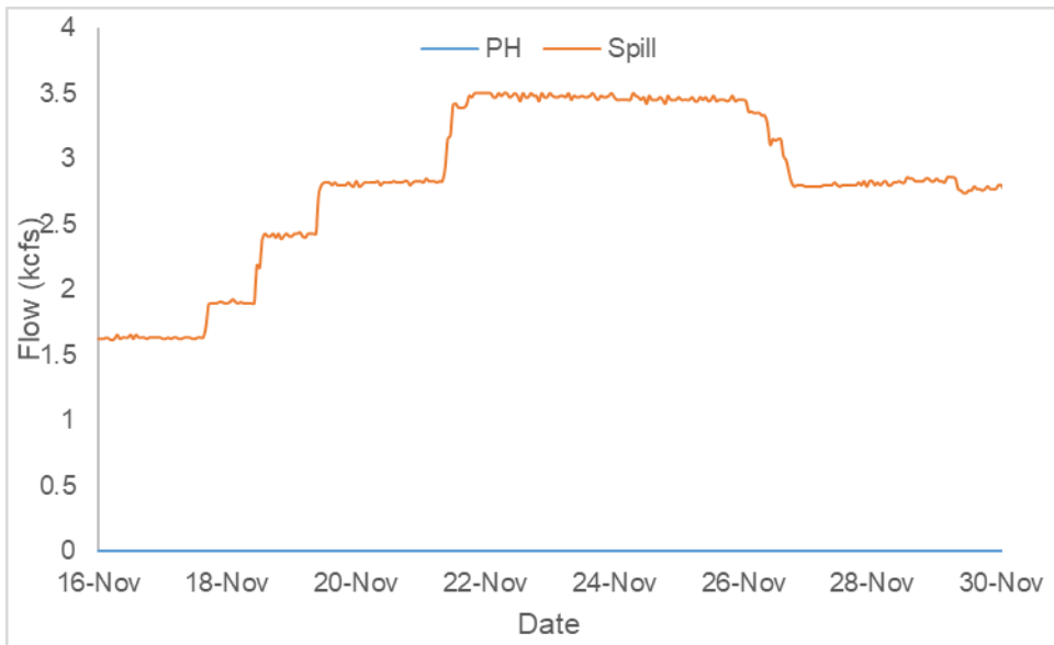
Figure 35. Hourly Flows PWR vs. Spill (Dexter Dam).
