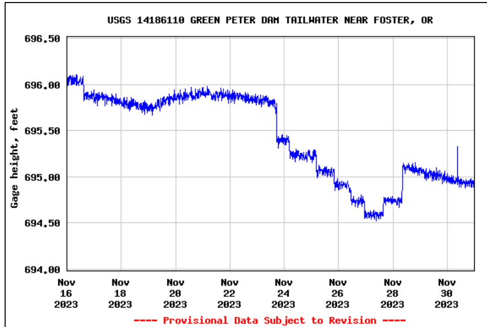
Figure 10. Gage Height (feet); below Green Peter Dam.
