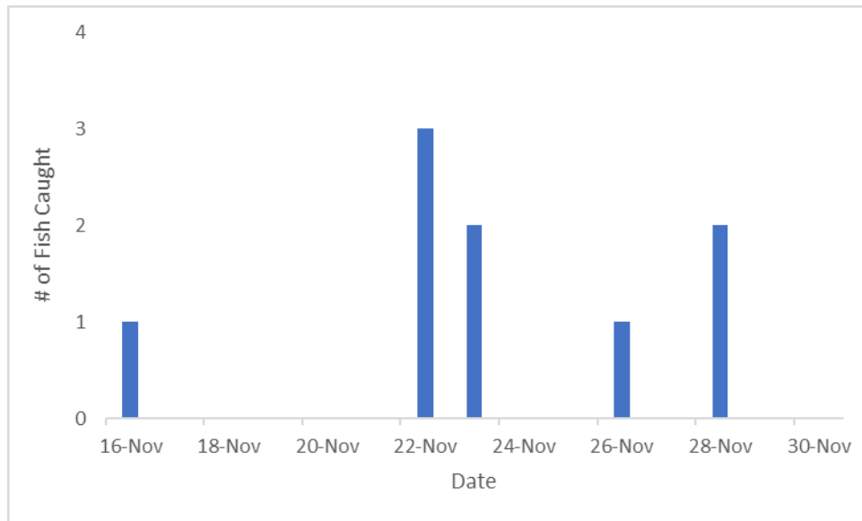
Figure 30. Chinook Captured Per Day 11/16/2023 to 11/30/2023 (Dexter Dam)
