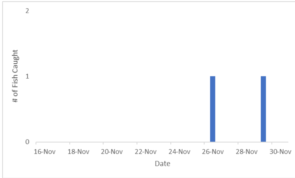
Figure 36. Chinook Captured Per Day 11/16/2023 to 11/30/2023 (Lookout Point Head of Reservoir).
