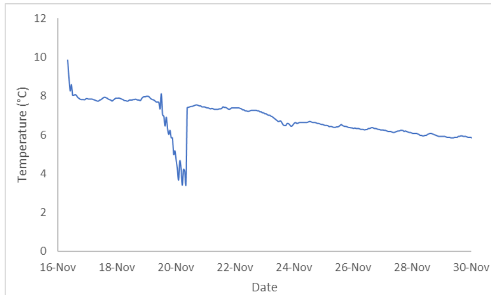
Figure 22. Temperature at RO RST (Cougar Dam).
