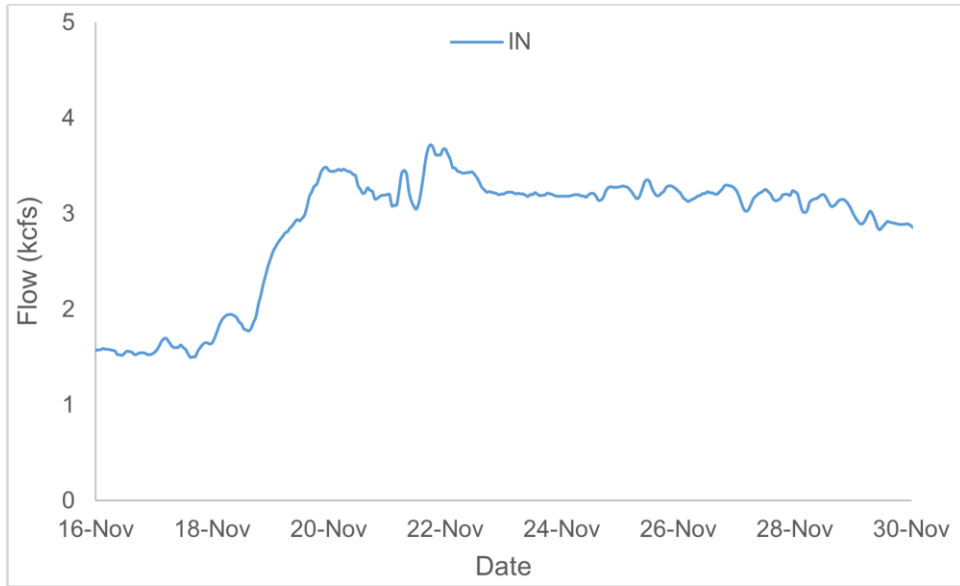
Figure 40. Hourly Flows (Lookout Point Head of Reservoir site).
