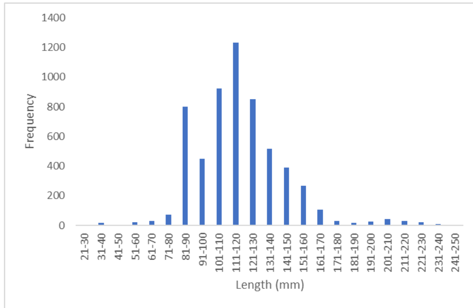
Figure 19. Length Frequency of Juvenile Chinook Sampled in 2023 (Cougar Dam).
