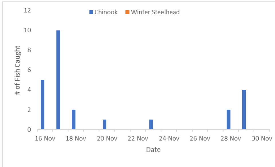
Figure 14. Chinook and Winter Steelhead Captured Per Day 11/16/2023 to 11/30/2023 (Foster Dam Head of Reservoir- South Santiam).
