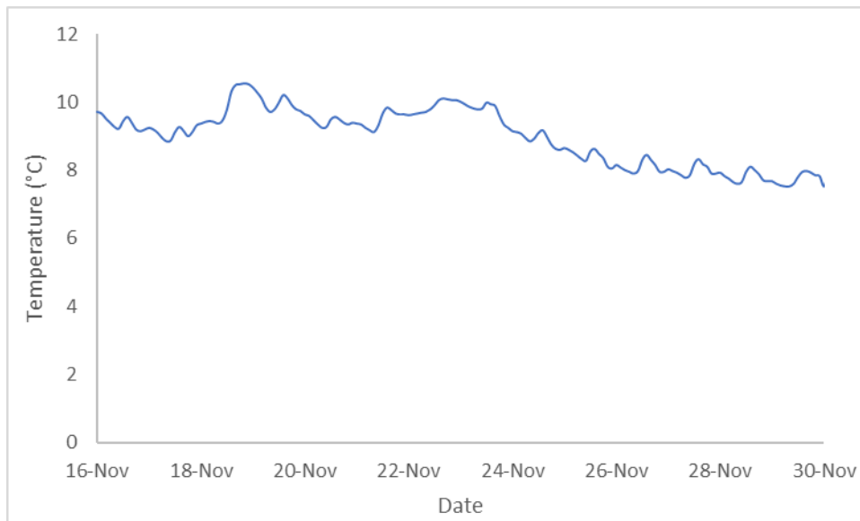
Figure 39. Temperature at RST (Lookout Point Head of Reservoir).
